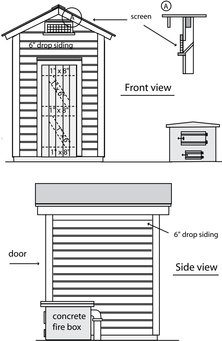
Fig. 10.15.1 General view
