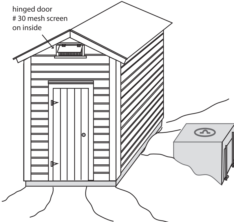
Fig. 11.18.1 General view.
